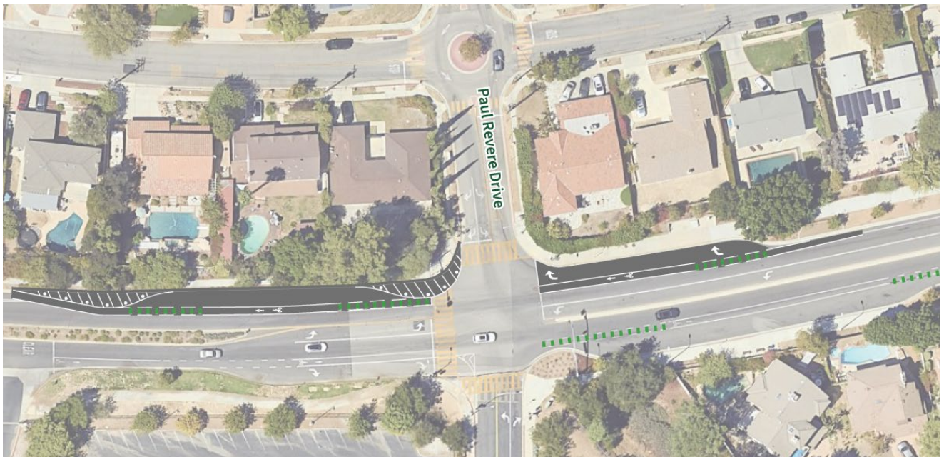
Figure 5.3 Class II Bike Lane Modifications on Mullholland Highway at Paul Revere Drive
