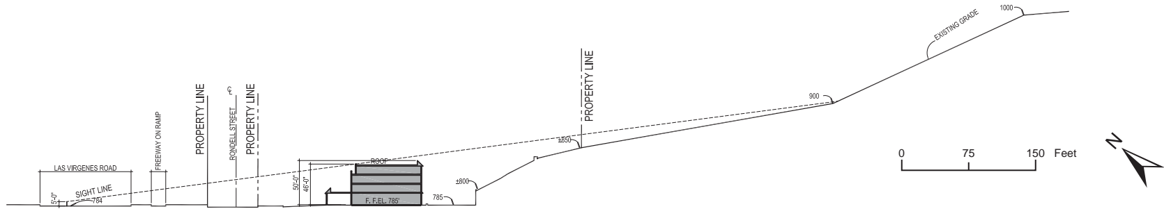
Section F-F
